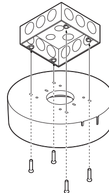
Type A : 2-Gang Handy Boxes / Switch Boxes
